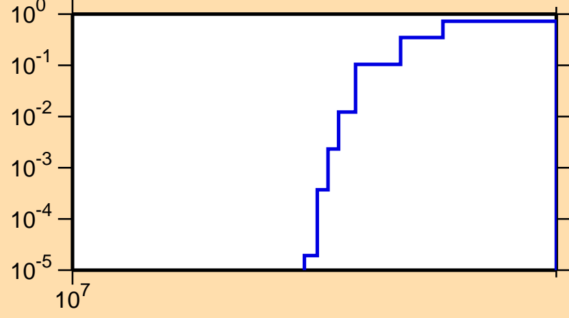
\sigma vs. E for ^{192}\text{Ir}(n,3n)
