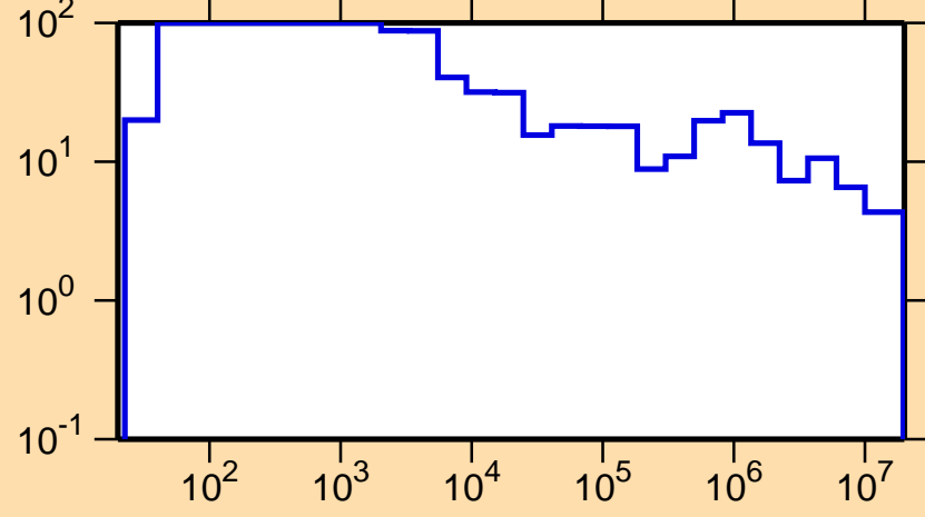
\Delta\sigma/\sigma vs. E for ^{192}\text{Ir}(n,\text{tot.})
