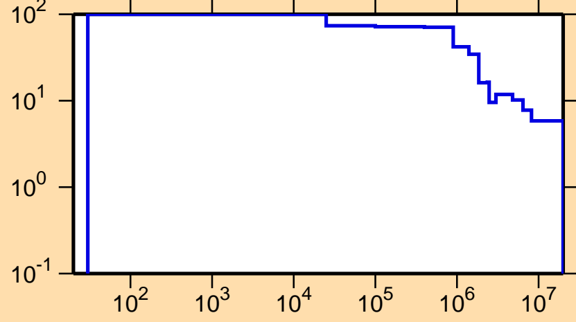
\Delta\sigma/\sigma vs. E for ^{192}\text{Ir}(n,\text{nonel.})
