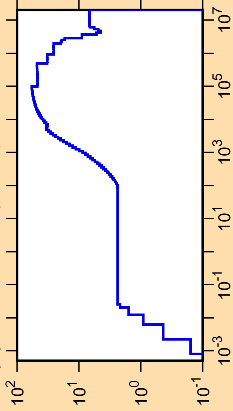
\Delta\mu/\mu vs. E for ^{193}\text{Ir}(\text{mt251})
