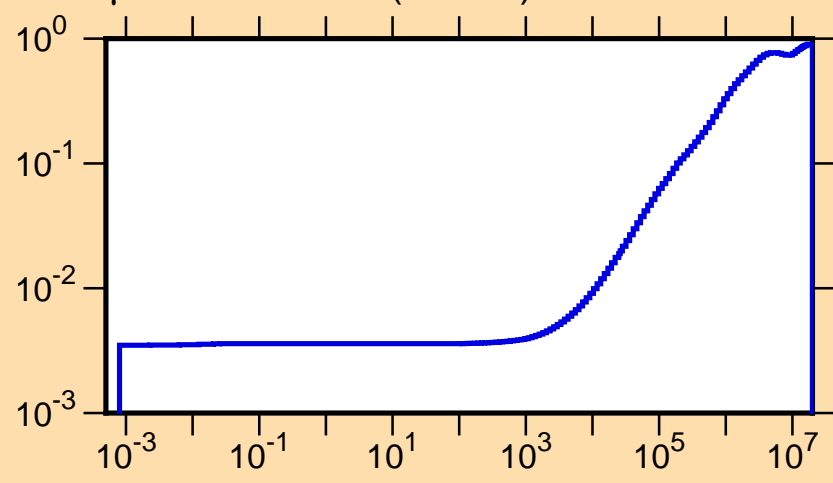
\mu vs. E for ^{193}\text{Ir}(\text{mt251})
