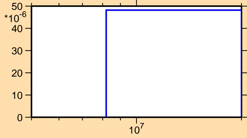
\sigma vs. E for ^{193}\text{Ir}(n,t)
