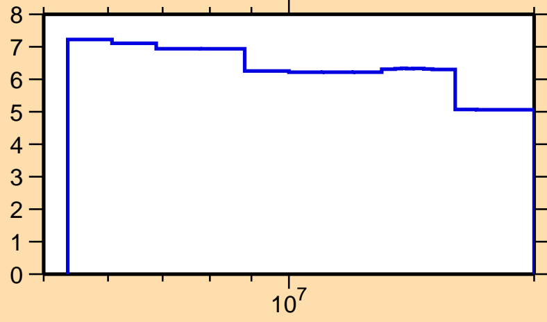
\Delta\sigma/\sigma vs. E for ^{194}\text{Ir}(n,\text{nonel.})
