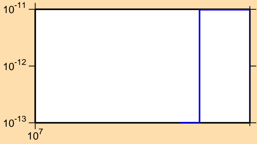
\sigma vs. E for ^{194}\text{Ir}(n,\text{He}3)
