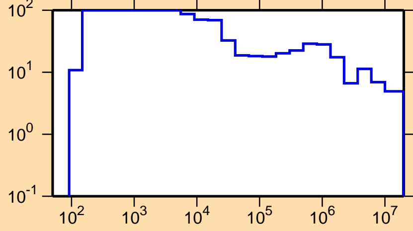
\Delta\sigma/\sigma vs. E for ^{194}\text{Ir}(n,\text{tot.})
