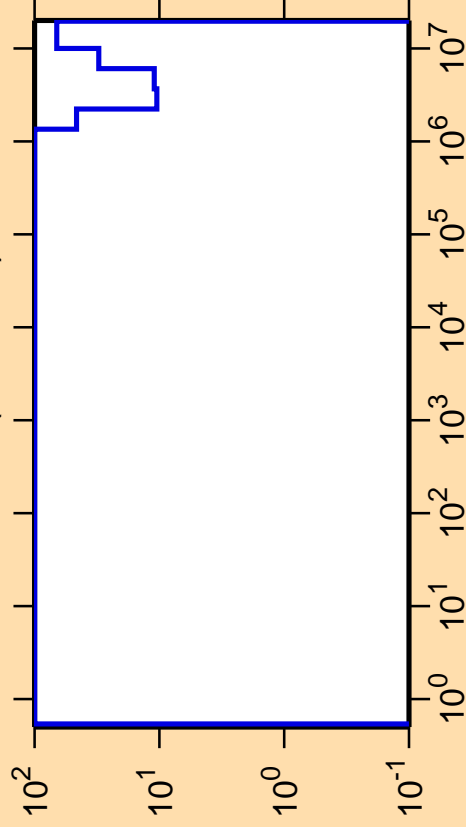
\Delta\sigma/\sigma vs. E for ^{194}\text{Ir}(n,n\text{cont.})
