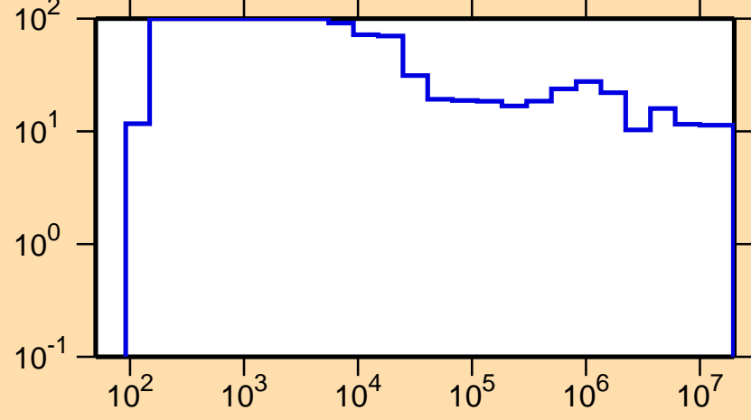
\Delta\sigma/\sigma vs. E for ^{194}\text{Ir}(n,\text{el.})
