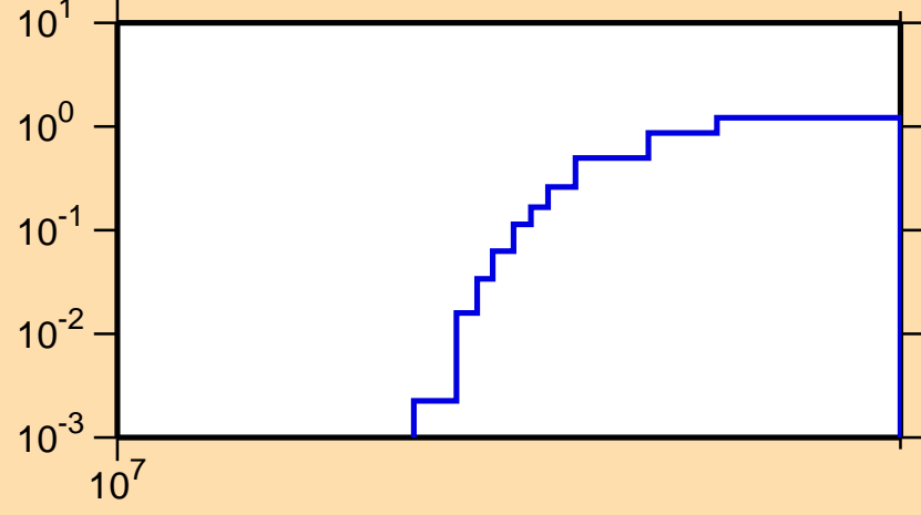
\sigma vs. E for ^{196}\text{Ir}(n,3n)
