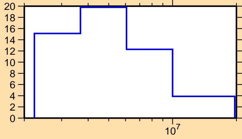
\Delta\sigma/\sigma vs. E for ^{196}\text{Ir}(n,el.)
