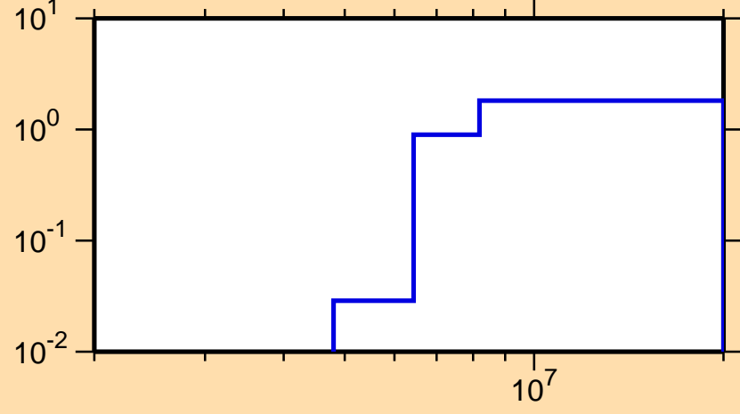
\sigma vs. E for ^{196}\text{Ir}(n,2n)
