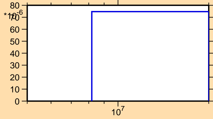
\sigma vs. E for ^{196}\text{Ir}(n,d)
