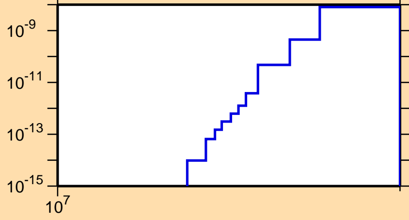
\sigma vs. E for ^{196}\text{Ir}(n,2n\alpha)
