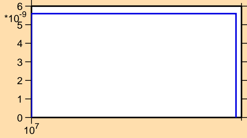
\sigma vs. E for ^{196}\text{Ir}(n,2np)
