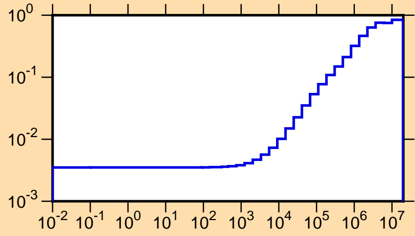
\mu vs. E for ^{197}\text{Ir}(\text{mt251})
