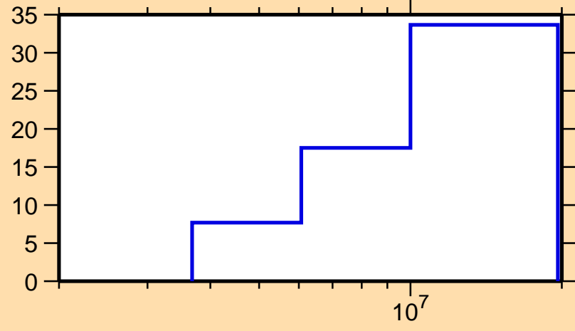
\Delta\sigma/\sigma vs. E for ^{197}\text{Ir}(n,ncont.)
