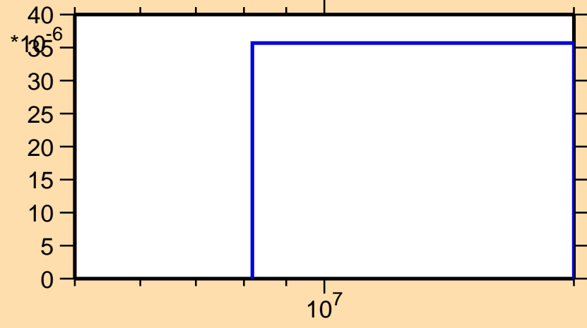
\sigma vs. E for ^{197}\text{Ir}(n,np)
