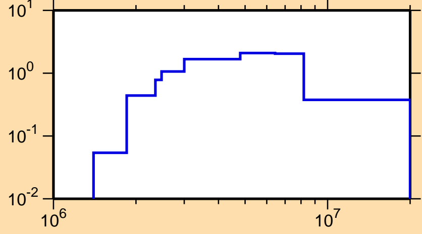
\sigma vs. E for ^{197}\text{Ir}(n,n\text{cont.})
