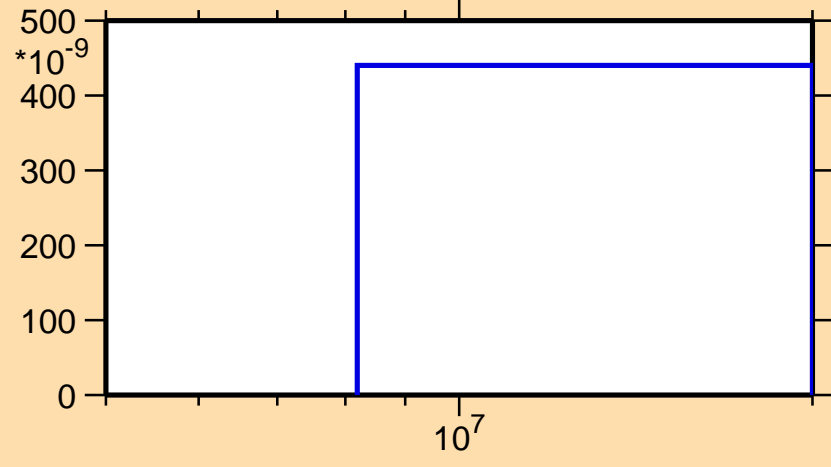
\sigma vs. E for ^{197}\text{Ir}(n,\alpha)
