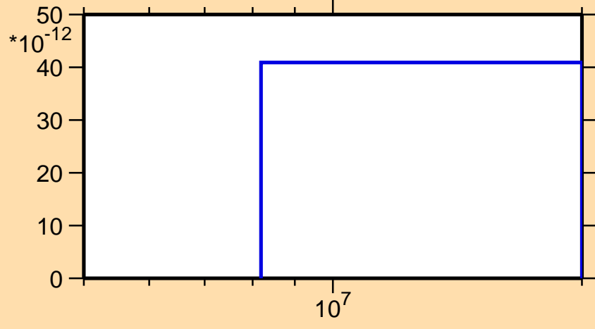
\sigma vs. E for ^{197}\text{Ir}(n,2np)
