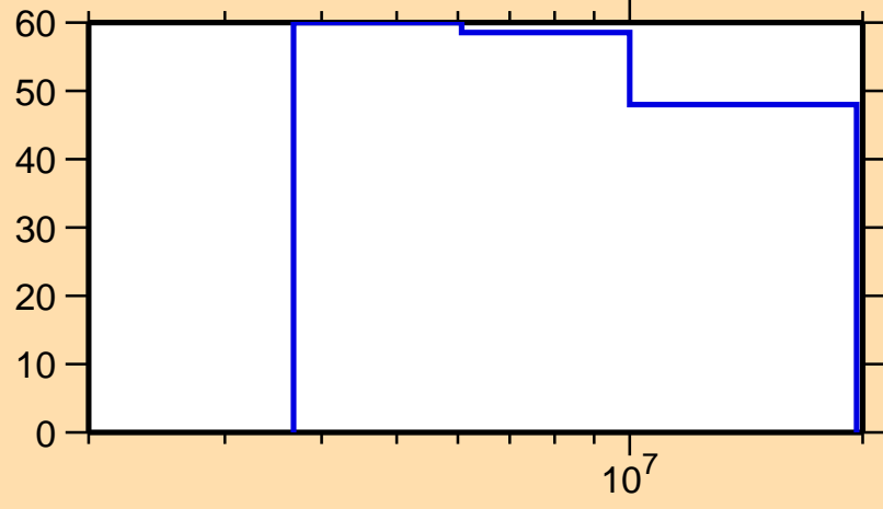
\Delta\sigma/\sigma vs. E for ^{197}\text{Ir}(n,p)
