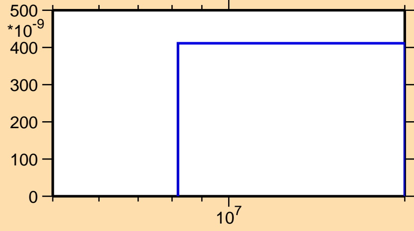
\sigma vs. E for ^{197}\text{Ir}(n,\alpha)
