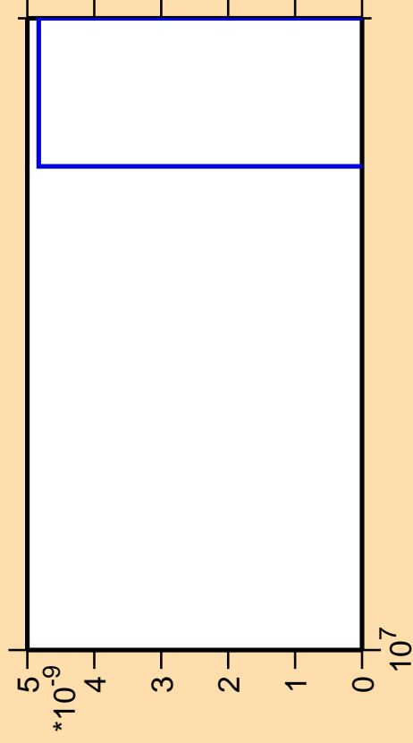
\Delta\sigma/\sigma vs. E for ^{198}\text{Ir}(\text{mt } 42)
