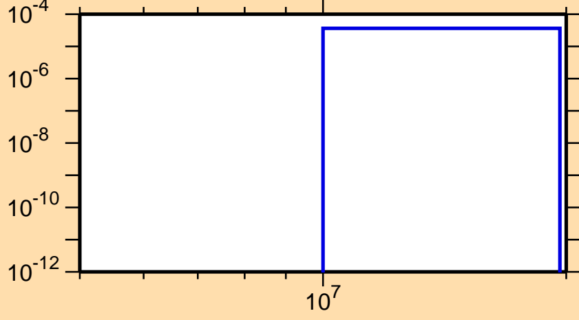
\sigma vs. E for ^{198}\text{Ir}(n,np)
