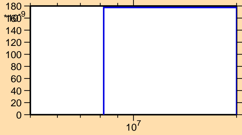
\sigma vs. E for ^{198}\text{Ir}(n,\alpha)
