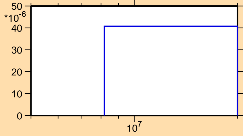
\sigma vs. E for ^{198}\text{Ir}(n,d)
