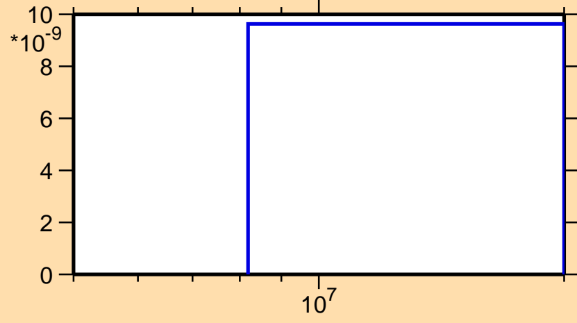
\sigma vs. E for ^{198}\text{Ir}(n,\text{nd})
