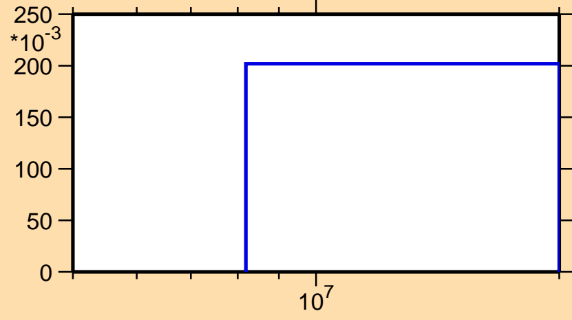
\sigma vs. E for ^{198}\text{Ir}(n,3n)
