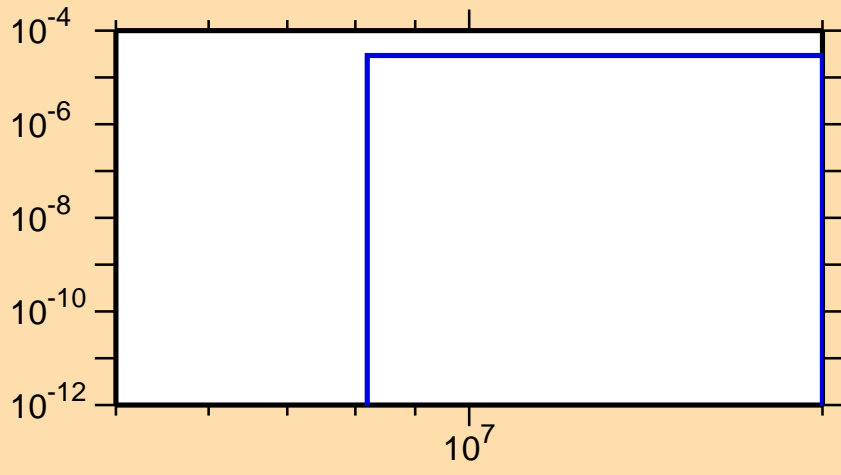
\sigma vs. E for ^{198}\text{Ir}(n,np)
