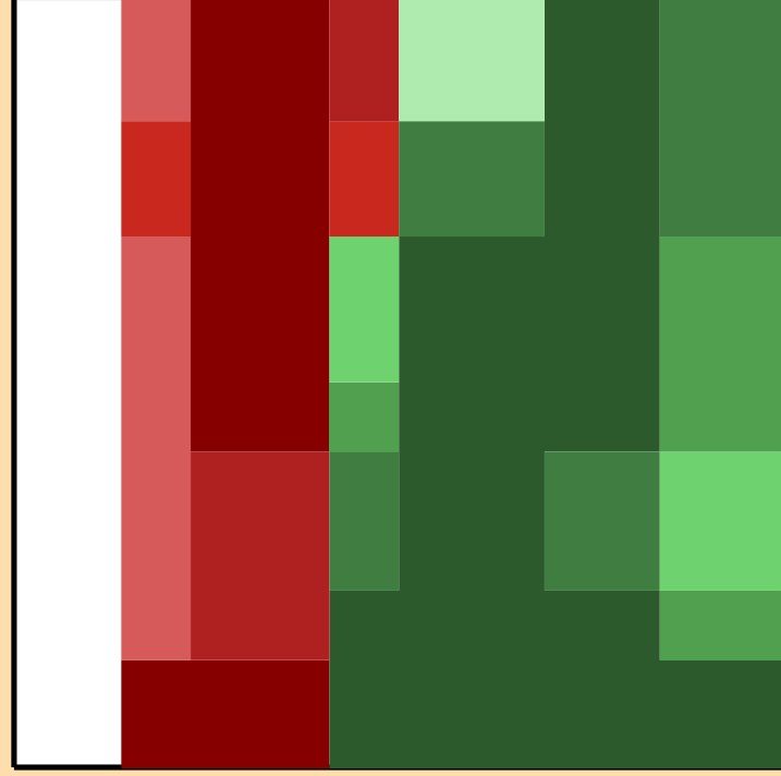
\Delta\sigma/\sigma vs. E for ^{199}\text{Ir}(n,2n)
