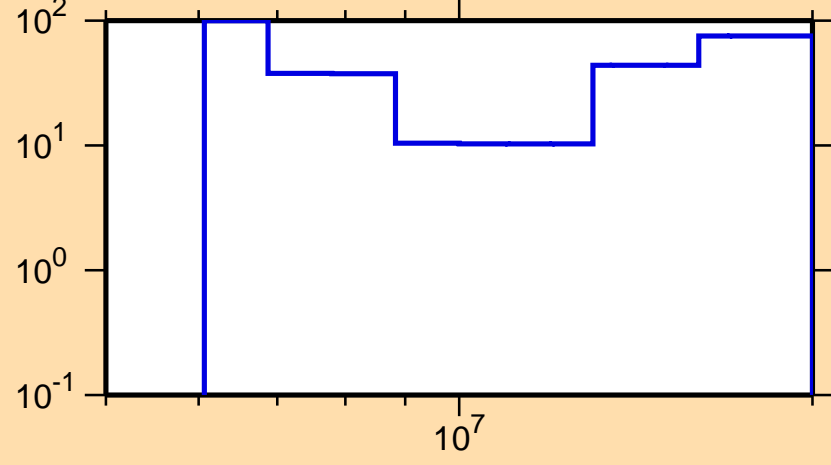
\Delta\sigma/\sigma vs. E for ^{199}\text{Ir}(n,2n)
