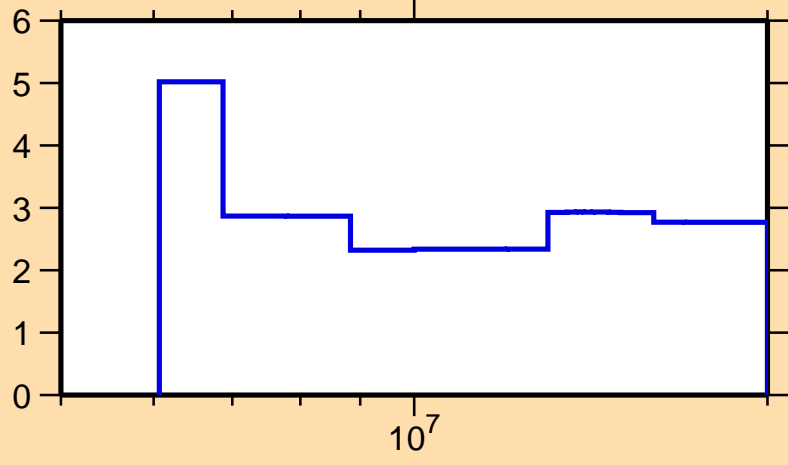
\Delta\sigma/\sigma vs. E for ^{199}\text{Ir}(n,\text{nonel.})
