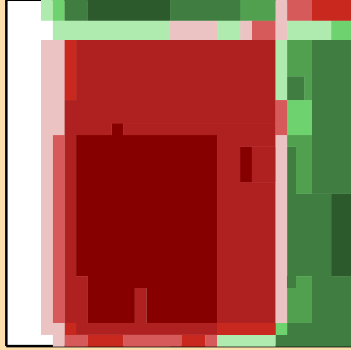
\Delta\sigma/\sigma vs. E for ^{199}\text{Ir}(n,n\text{cont.})
