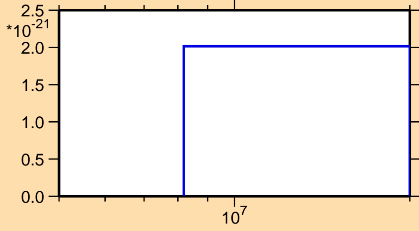
\sigma vs. E for ^{199}\text{Ir} (mt 42)
