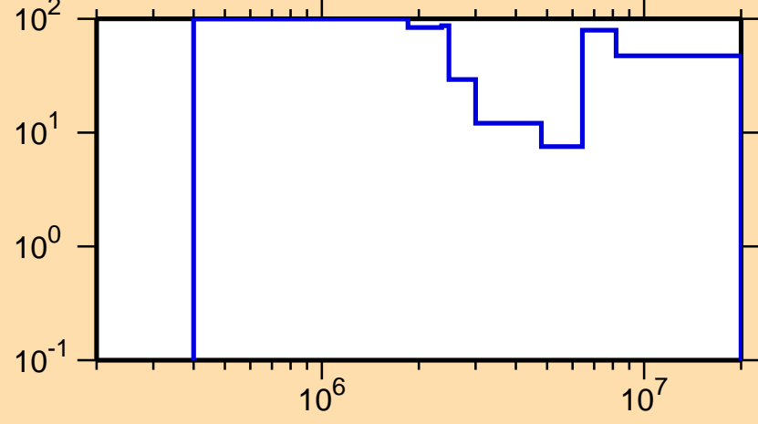
\Delta\sigma/\sigma vs. E for ^{199}\text{Ir}(n,n\text{cont.})
