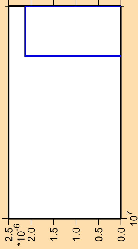
\Delta\sigma/\sigma vs. E for ^{200}\text{Ir} (mt 42)
