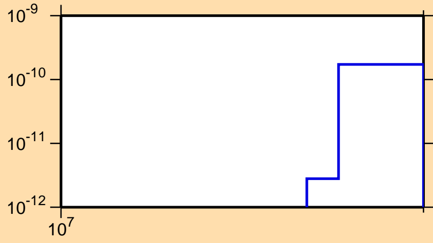
\sigma vs. E for ^{200}\text{Ir}(n,2n\alpha)
