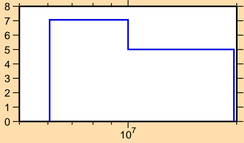
\Delta\sigma/\sigma vs. E for ^{200}\text{Ir}(n,\text{tot.})
