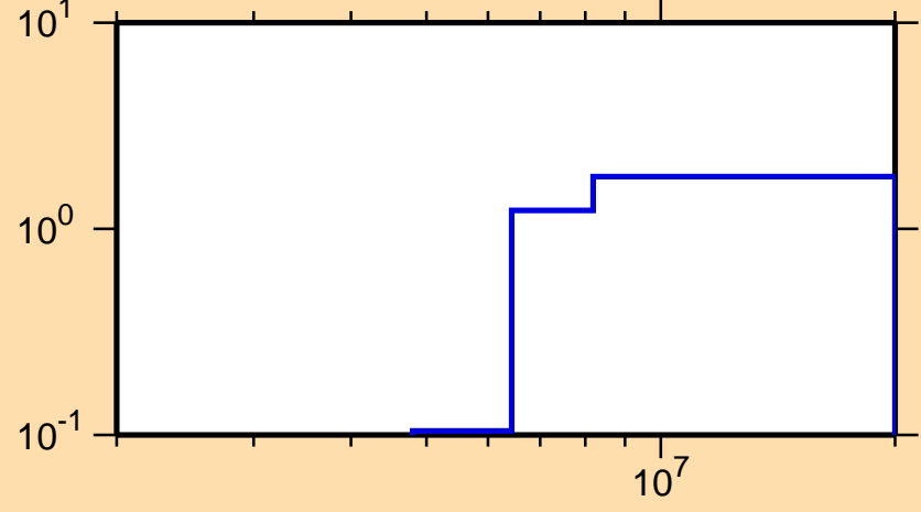
\sigma vs. E for ^{200}\text{Ir}(n,2n)
