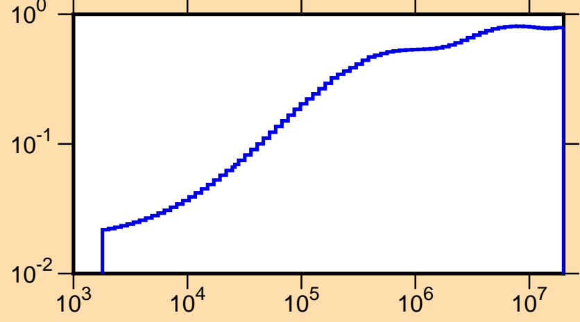
\mu vs. E for ^{37}\text{K}(\text{mt251})
