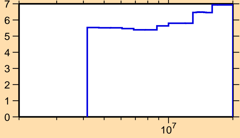
\Delta\sigma/\sigma vs. E for ^{37}\text{K}(n,n\text{onel.})
