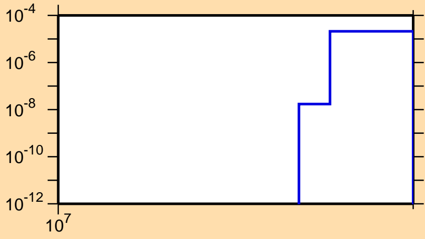
\sigma vs. E for ^{37}\text{K}(n,pt)
