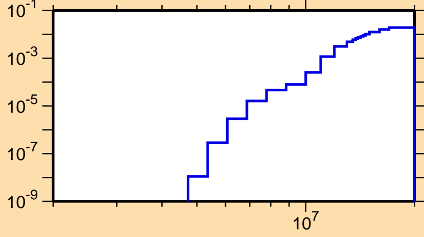
\sigma vs. E for ^{37}\text{K}(n,\text{He3})
