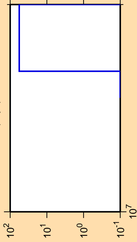
\Delta\sigma/\sigma vs. E for ^{37}\text{K}(n,pt)
