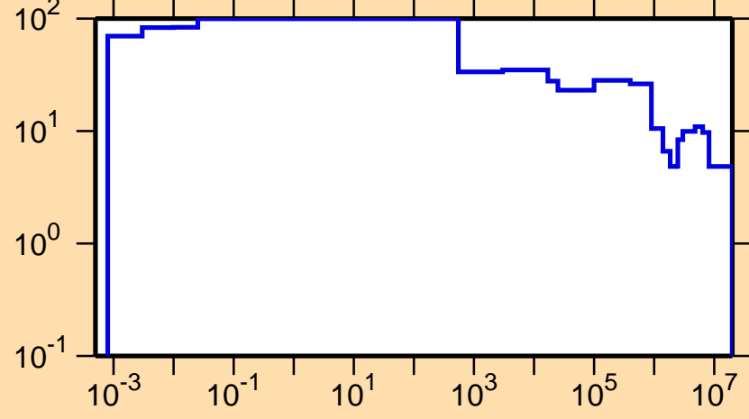
\Delta\sigma/\sigma vs. E for ^{37}\text{K}(n,\text{tot.})
