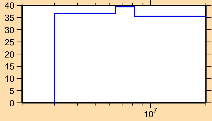
\Delta\sigma/\sigma vs. E for ^{37}\text{K}(n,n\text{cont.})
