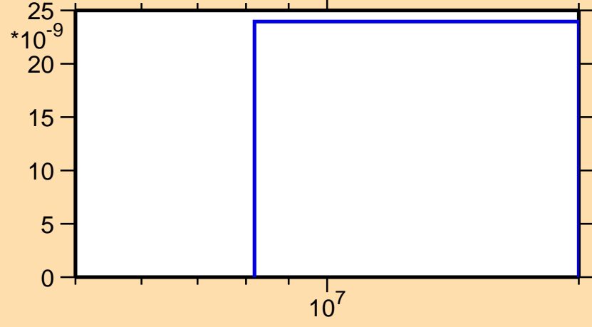
\sigma vs. E for ^{37}\text{K}(n,nd)
