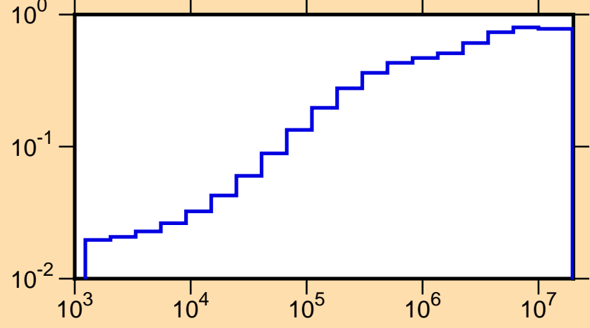
\mu vs. E for ^{38}\text{K}(\text{mt251})
