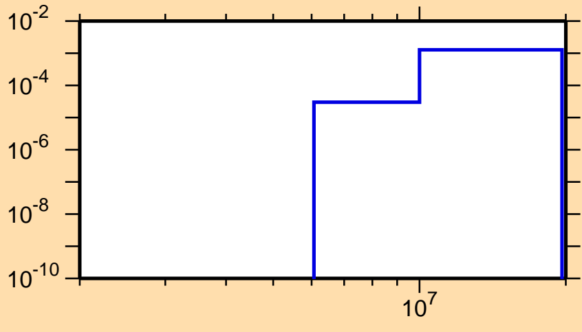
\sigma vs. E for ^{38}\text{K}(n,t)
