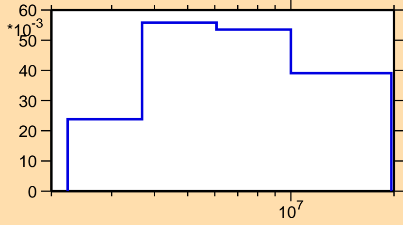
\sigma vs. E for ^{38}\text{K}(n,n_4)
