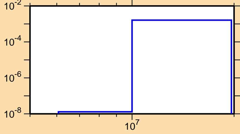
\sigma vs. E for ^{38}\text{K}(n,\text{He}3)
