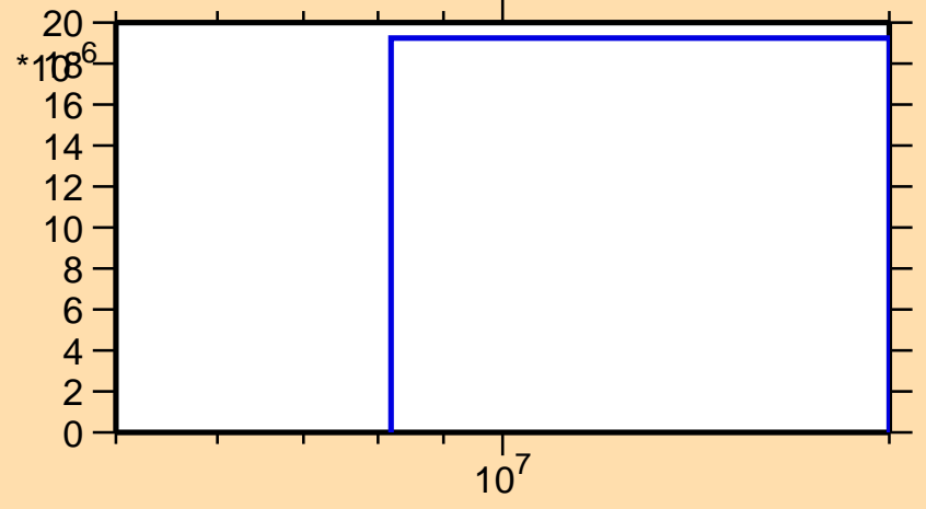
\sigma vs. E for ^{38}\text{K}(\text{mt117})
