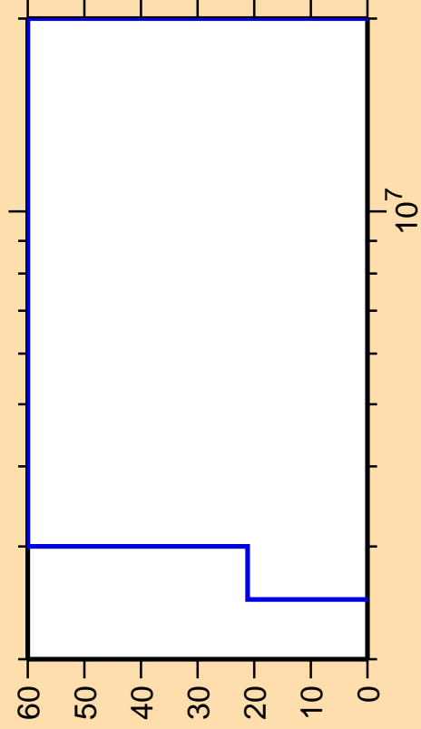
\Delta\sigma/\sigma vs. E for ^{38}\text{K}(n,d)
