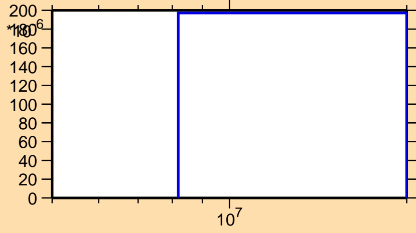
\sigma vs. E for ^{38}\text{K}(n,nd)
