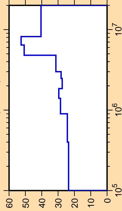
\Delta\sigma/\sigma vs. E for ^{38}\text{K}(n,\text{inel.})
