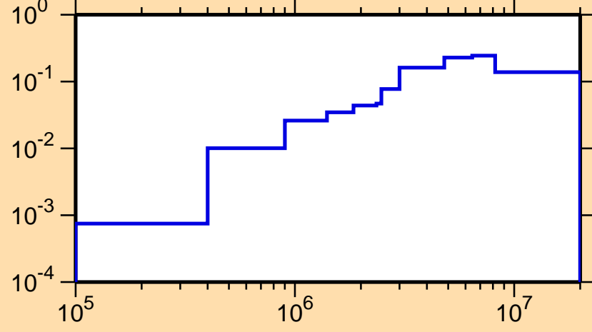
\sigma vs. E for ^{38}\text{K}(n,\text{inel.})
