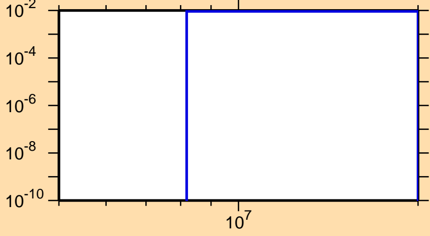
\sigma vs. E for ^{38}\text{K}(n,n\alpha)
