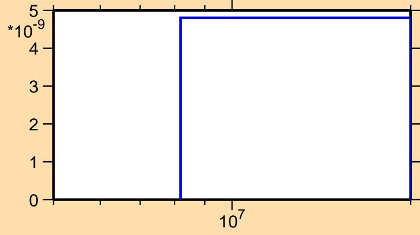
\sigma vs. E for ^{38}\text{K} (mt 34)
