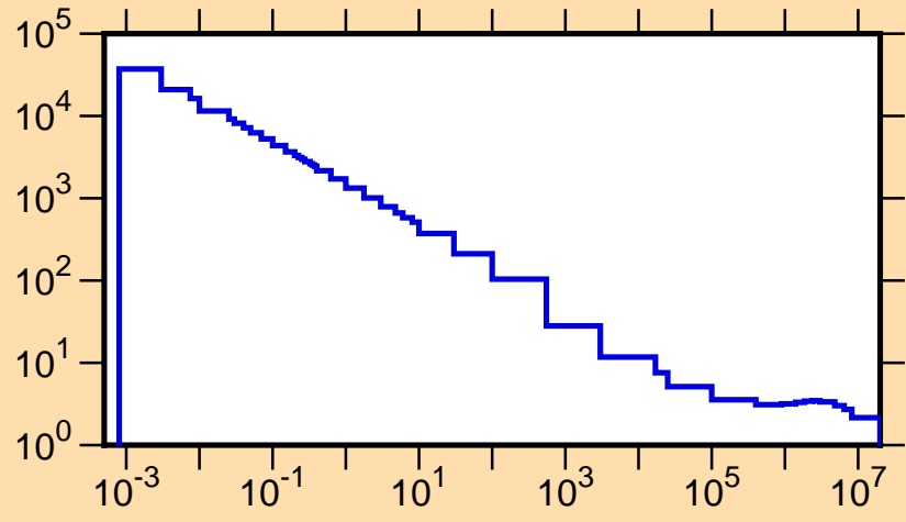
\sigma vs. E for ^{38}\text{K}(n,\text{tot.})
