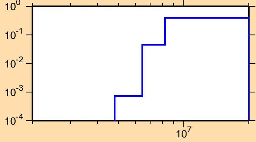
\sigma vs. E for ^{38}\text{K}(n,np)
