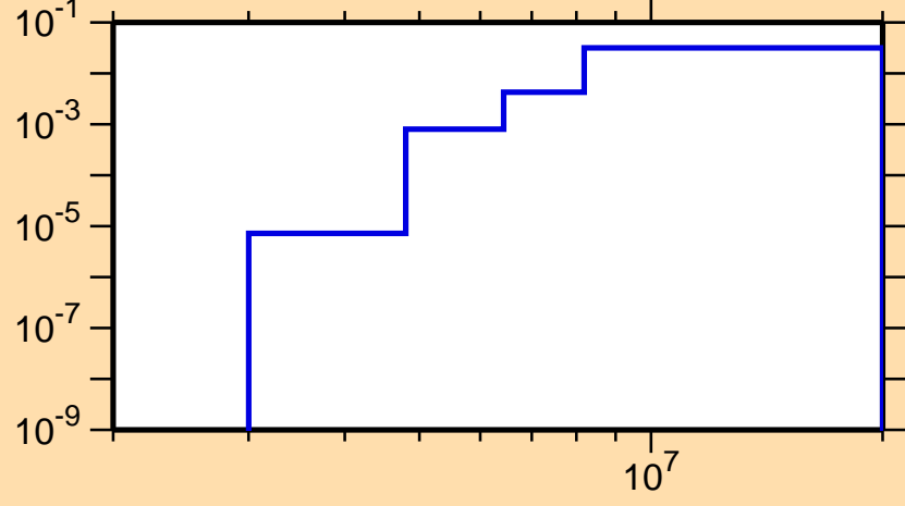
\sigma vs. E for ^{38}\text{K}(n,d)
