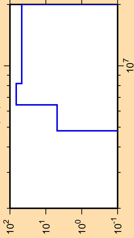
\Delta\sigma/\sigma vs. E for ^{38}\text{K}(n,t)
