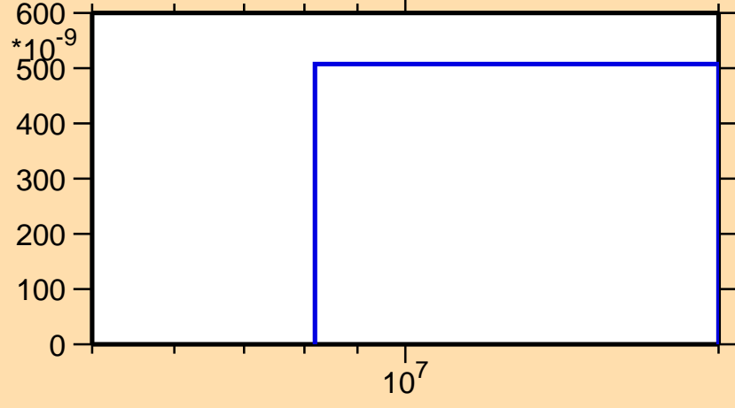
\sigma vs. E for ^{38}\text{K}(n,\text{pt})
