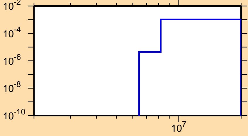
\sigma vs. E for ^{38}\text{K}(n,t)
