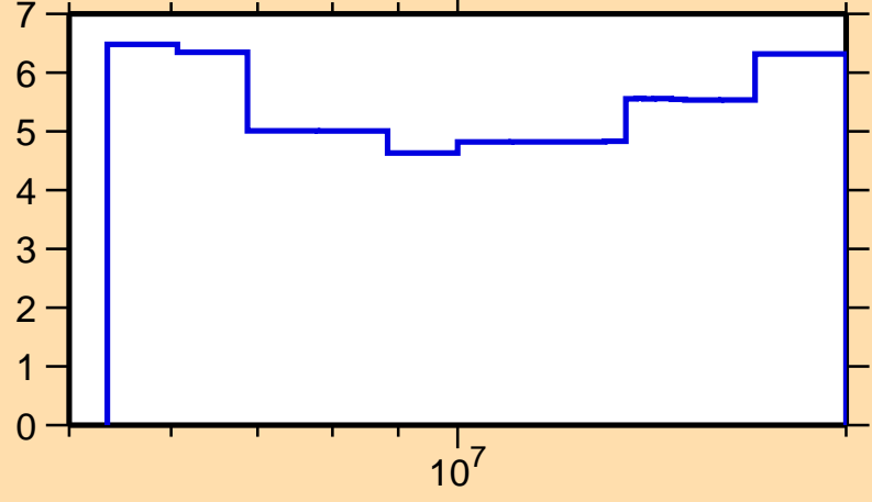
\Delta\sigma/\sigma vs. E for ^{39}\text{K}(n,n\text{onel.})
