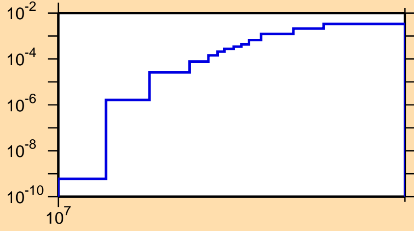
\sigma vs. E for ^{39}\text{K}(n,t)
