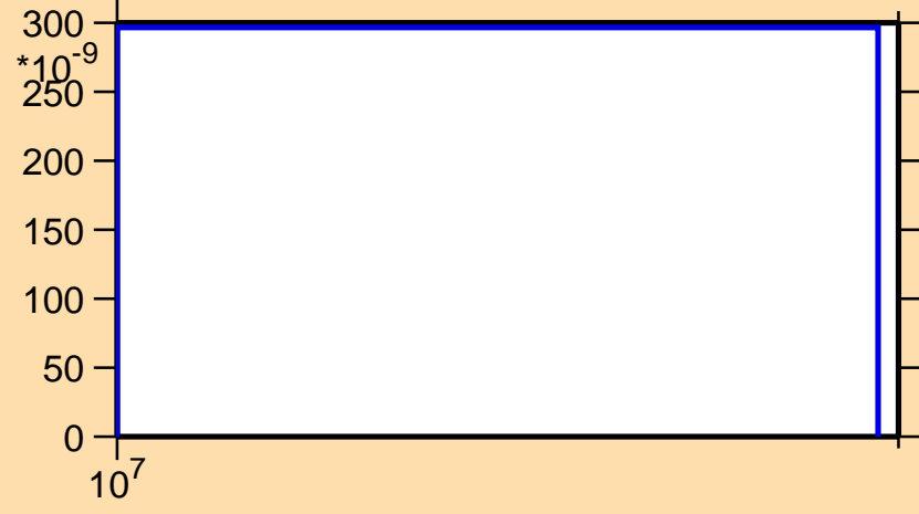
\sigma vs. E for ^{39}\text{K}(n,\text{pd})
