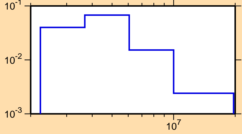
\sigma vs. E for ^{39}\text{K}(n,n_1)
