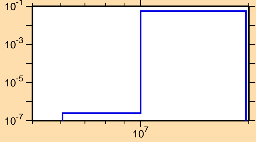
\sigma vs. E for ^{39}\text{K}(n,n\alpha)
