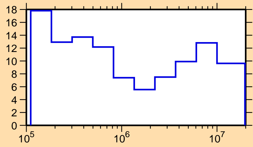
\Delta\sigma/\sigma vs. E for ^{39}\text{K}(n,el.)
