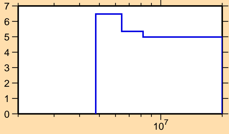
\Delta\sigma/\sigma vs. E for ^{39}\text{K}(n,n\text{onel.})
