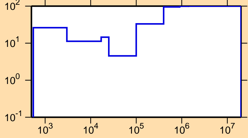
\Delta\sigma/\sigma vs. E for ^{39}\text{K}(n,\gamma)
