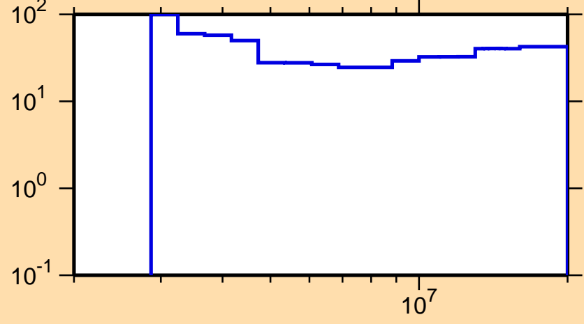
\Delta\sigma/\sigma vs. E for ^{40}\text{K}(n,ncont.)
