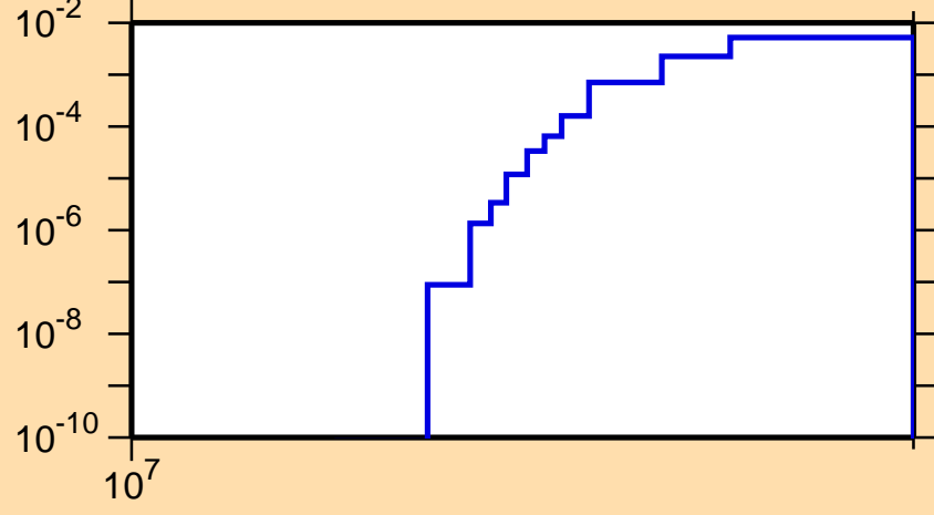
\sigma vs. E for ^{40}\text{K}(n,nd)
