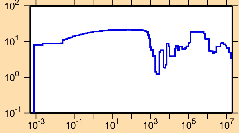
\Delta\sigma/\sigma vs. E for ^{41}\text{K}(n,\text{tot.})
