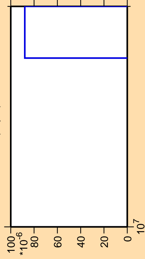
\Delta\sigma/\sigma vs. E for ^{41}\text{K}(n,\text{pd})
