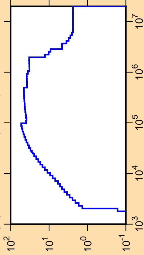
\Delta\mu/\mu vs. E for ^{42}\text{K}(\text{mt251})
