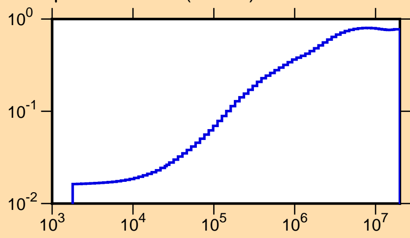
\mu vs. E for ^{42}\text{K}(\text{mt251})
