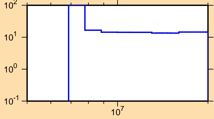
\Delta\sigma/\sigma vs. E for ^{42}\text{K}(n,2n)
