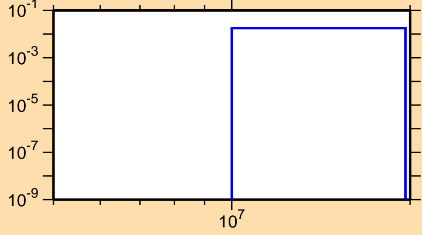
\sigma vs. E for ^{42}\text{K}(n,n\alpha)
