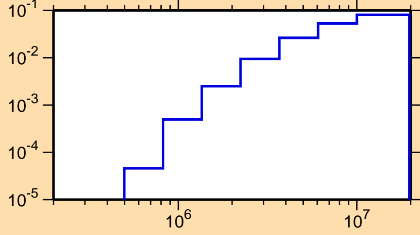
\sigma vs. E for ^{42}\text{K}(n,p)
