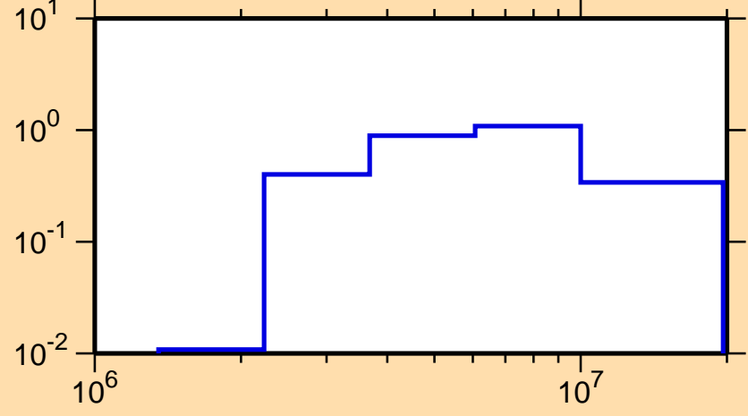
\sigma vs. E for ^{42}\text{K}(n,n\text{cont.})
