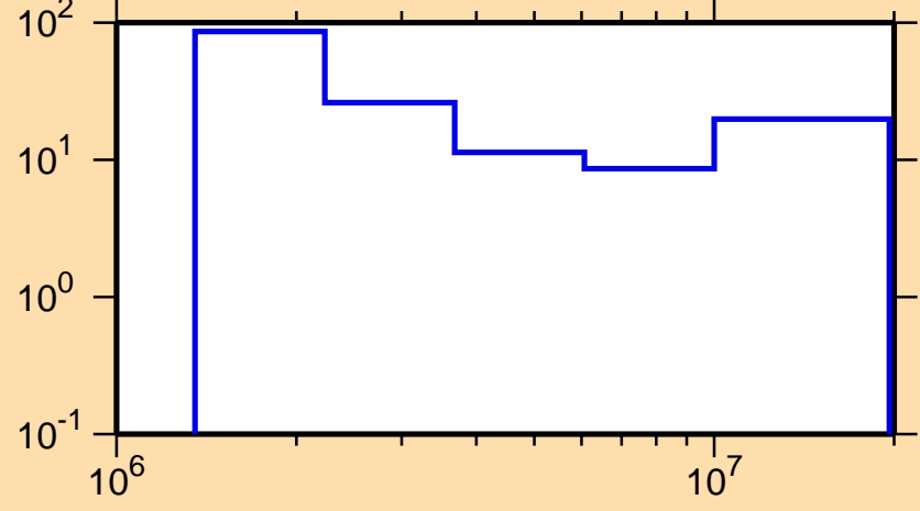
\Delta\sigma/\sigma vs. E for ^{42}\text{K}(n,n\text{cont.})
