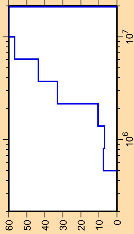
\Delta\sigma/\sigma vs. E for ^{42}\text{K}(n,n_4)
