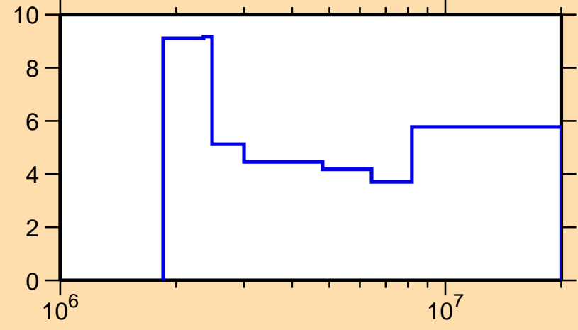
\Delta\sigma/\sigma vs. E for ^{42}\text{K}(n,n\text{onel.})
