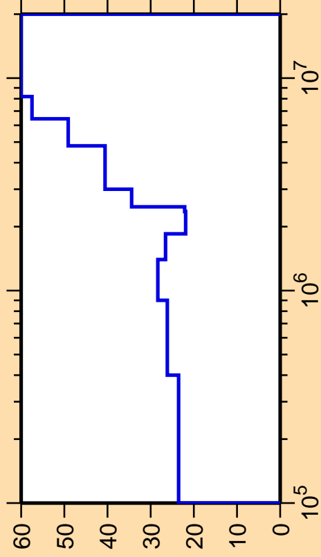
\Delta\sigma/\sigma vs. E for ^{42}\text{K}(n,n_2)
