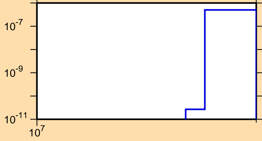
\sigma vs. E for ^{43}\text{K}(n,nt)
