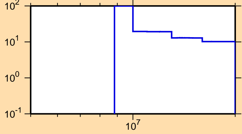
\Delta\sigma/\sigma vs. E for ^{43}\text{K}(n,2n)
