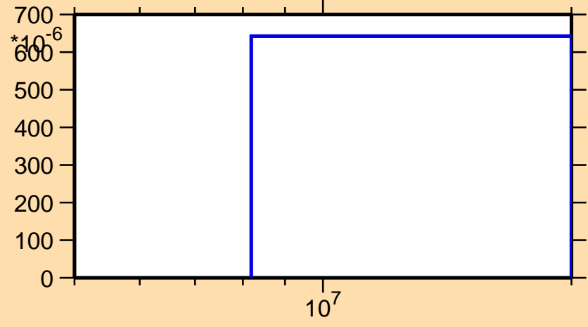
\sigma vs. E for ^{43}\text{K}(n,n\alpha)
