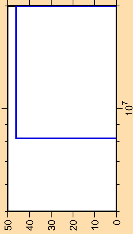
\Delta\sigma/\sigma vs. E for ^{43}\text{K}(n,np)
