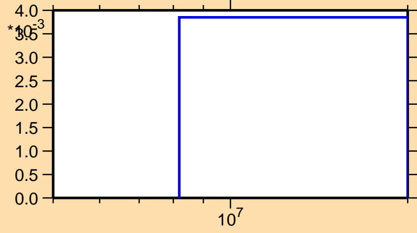
\sigma vs. E for ^{43}\text{K}(n,np)
