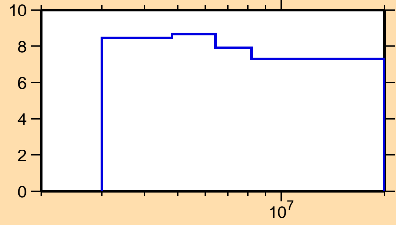
\Delta\sigma/\sigma vs. E for ^{43}\text{K}(n,n\text{onel.})
