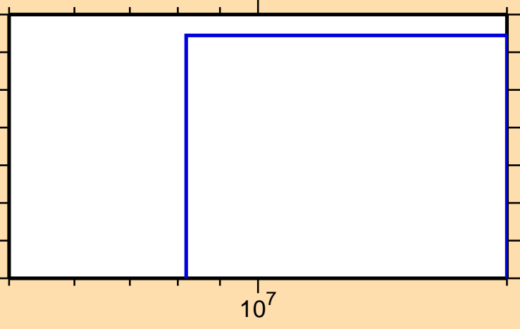
\sigma vs. E for ^{43}\text{K}(n,t)
