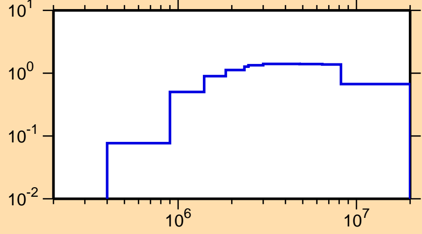
\sigma vs. E for ^{43}\text{K}(n,\text{inel.})
