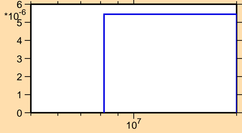
\sigma vs. E for ^{43}\text{K}(n,3n)
