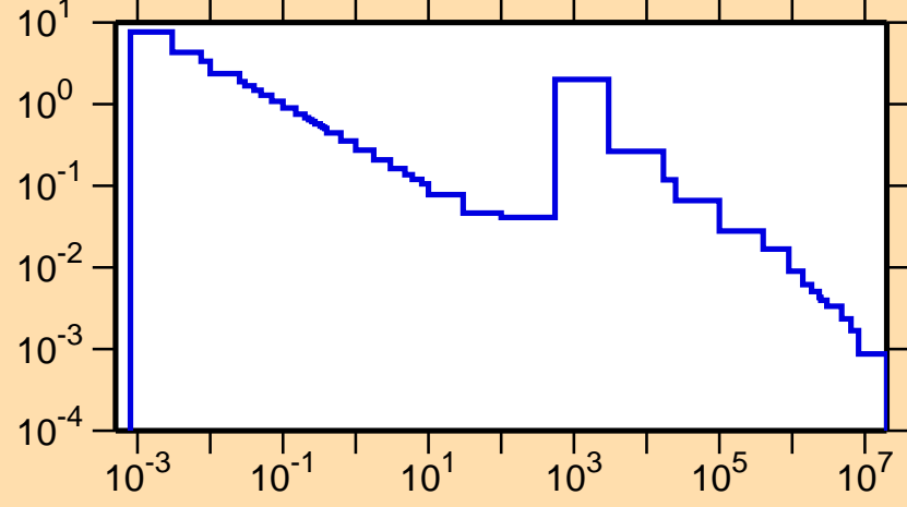
\sigma vs. E for ^{43}\text{K}(n,\gamma)
