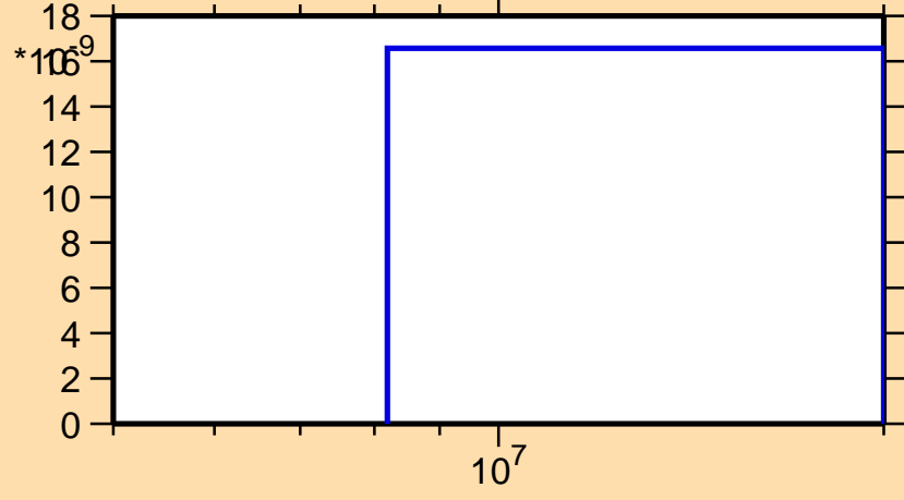
\sigma vs. E for ^{43}\text{K}(n,nd)
