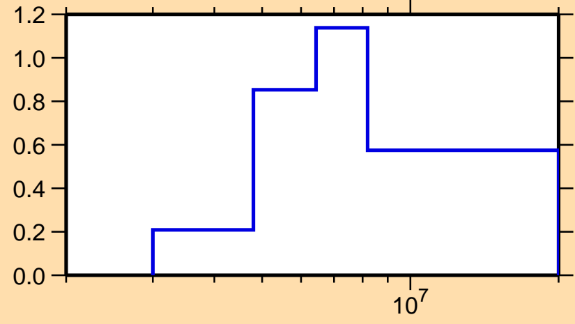
\sigma vs. E for ^{43}\text{K}(n,n\text{cont.})
