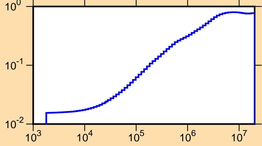
\mu vs. E for ^{44}\text{K}(\text{mt251})
