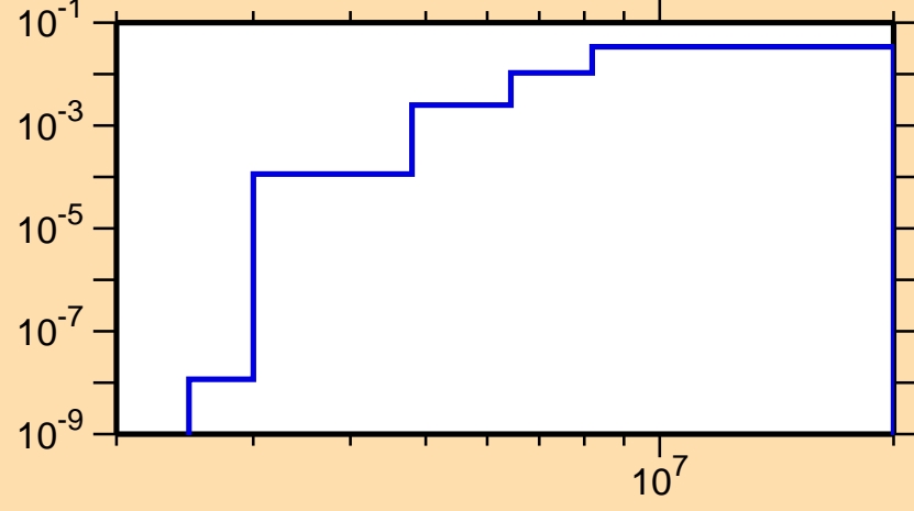
\sigma vs. E for ^{44}\text{K}(n,p)
