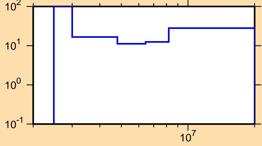
\Delta\sigma/\sigma vs. E for ^{44}\text{K}(n,n\text{cont.})
