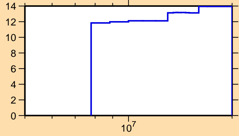
\Delta\sigma/\sigma vs. E for ^{45}\text{K}(n,n\text{nonel.})
