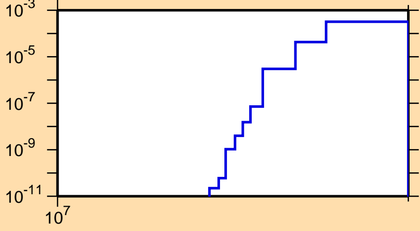
\sigma vs. E for ^{45}\text{K}(n,\alpha)
