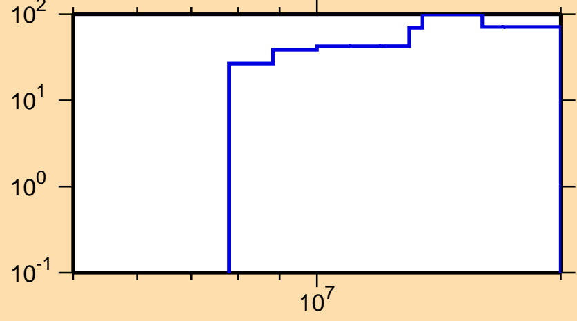
\Delta\sigma/\sigma vs. E for ^{45}\text{K}(n,n_1)
