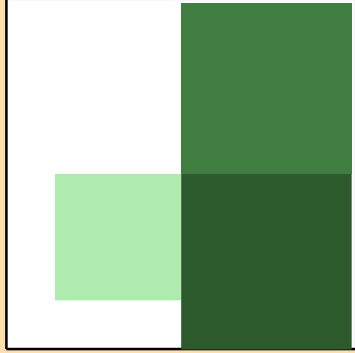
\Delta\sigma/\sigma vs. E for ^{45}\text{K}(n,n\text{cont.})
