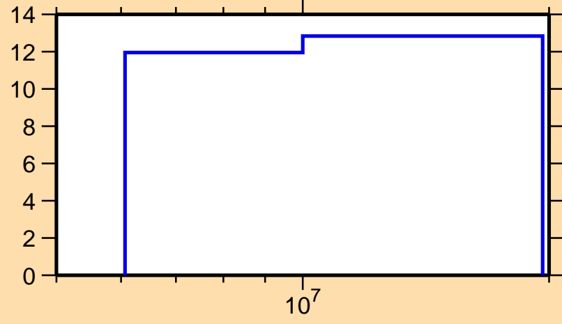
\Delta\sigma/\sigma vs. E for ^{45}\text{K}(n,n\text{onel.})
