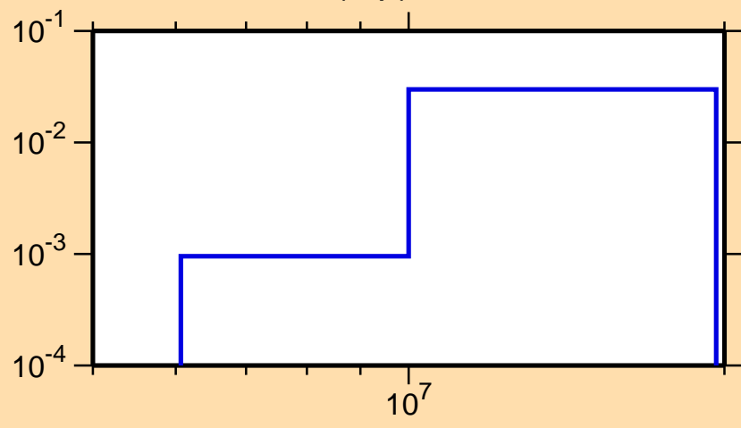
\sigma vs. E for ^{45}\text{K}(n,p)
