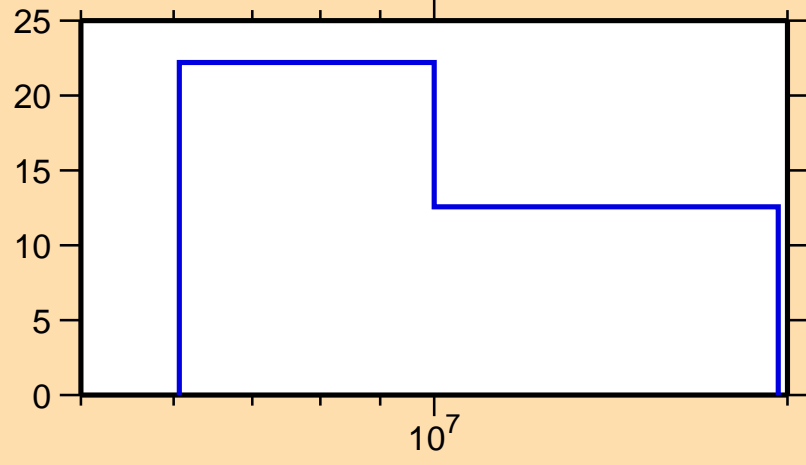
\Delta\sigma/\sigma vs. E for ^{45}\text{K}(n,el.)
