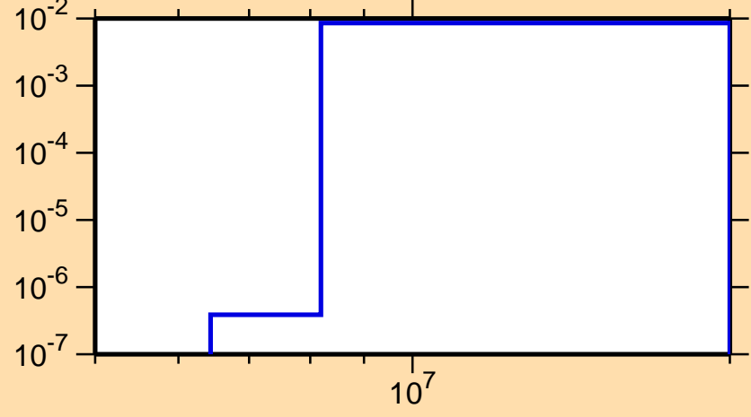
\sigma vs. E for ^{45}\text{K}(n,n\text{cont.})
