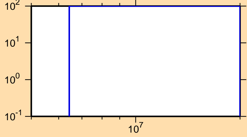
\Delta\sigma/\sigma vs. E for ^{45}\text{K}(n,ncont.)
