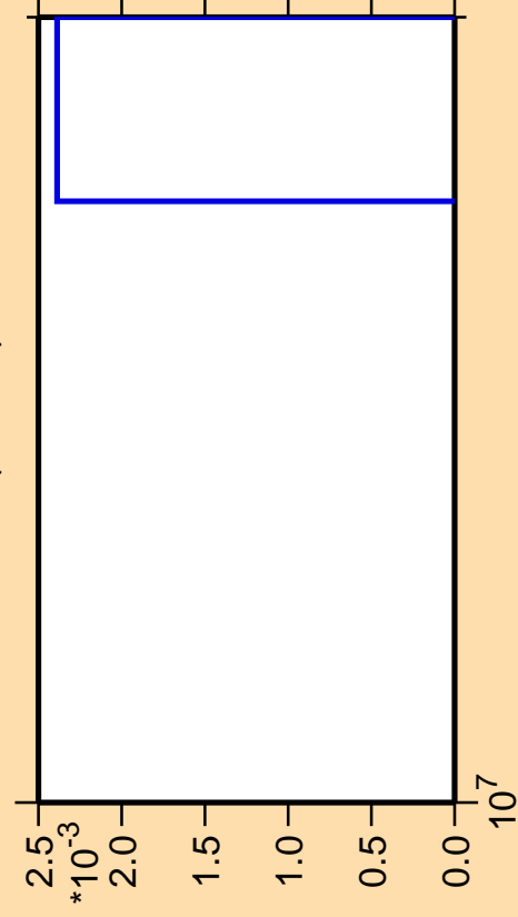
\Delta\sigma/\sigma vs. E for ^{46}\text{K}(n,2n\alpha)
