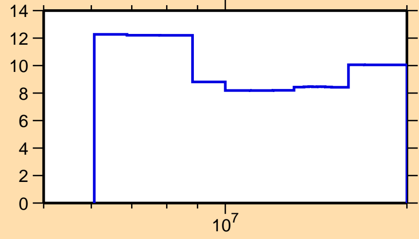
\Delta\sigma/\sigma vs. E for ^{46}\text{K}(n,n\text{onel.})
