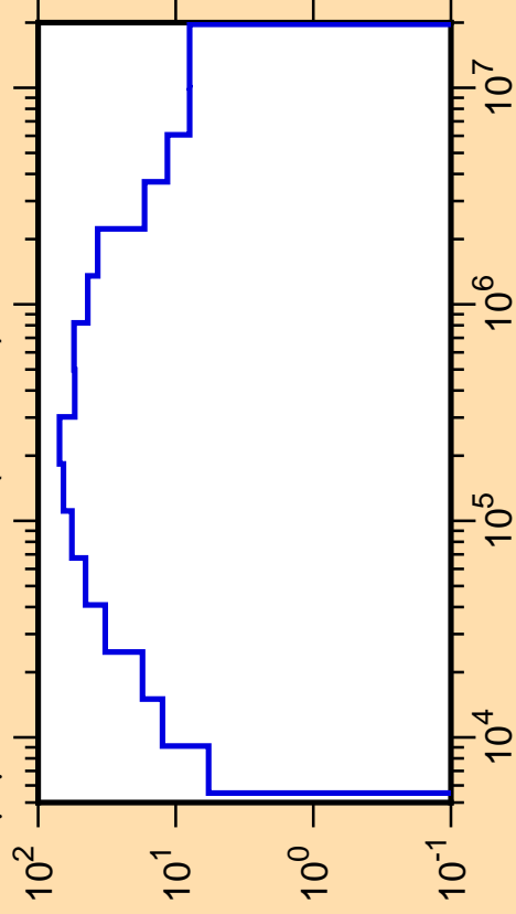
\Delta\mu/\mu vs. E for ^{46}\text{K}(\text{mt251})
