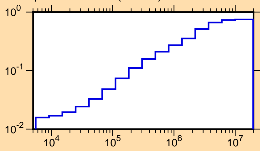
\mu vs. E for ^{46}\text{K}(\text{mt251})
