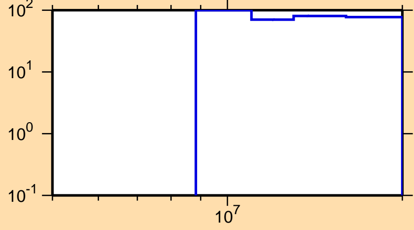
\Delta\sigma/\sigma vs. E for ^{47}\text{K}(n,p)
