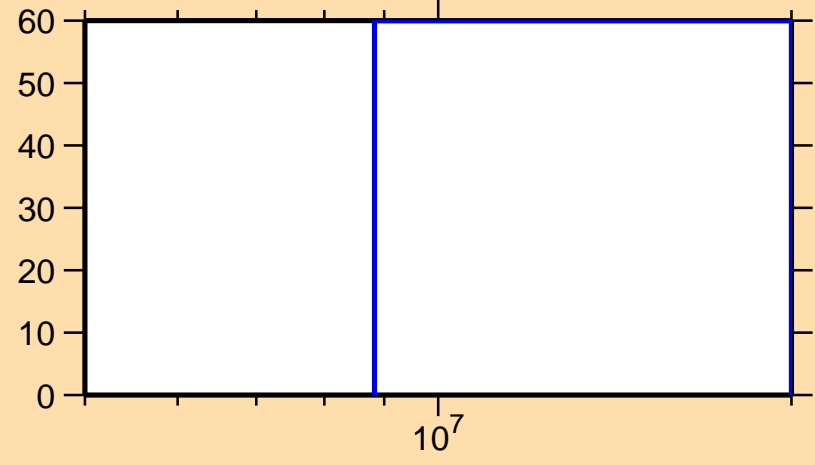
\Delta\sigma/\sigma vs. E for ^{47}\text{K}(n,n\text{cont.})
